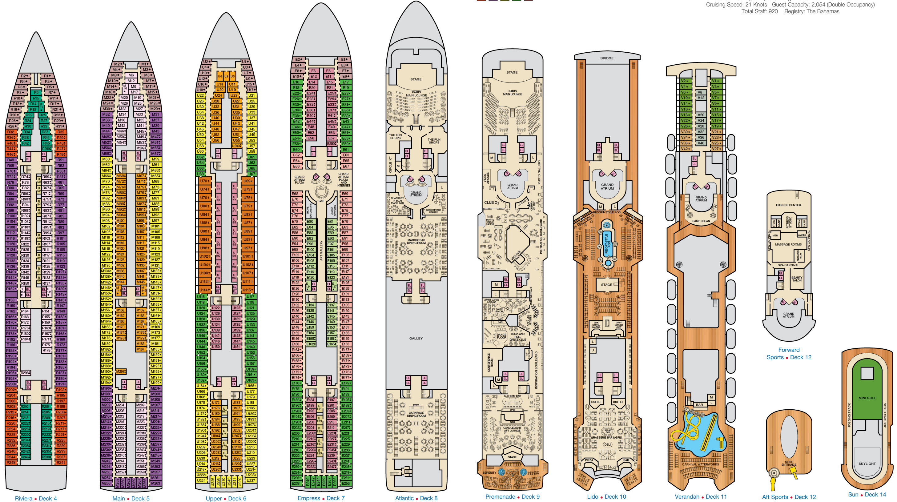
Riviera • Deck 4 Main • Deck 5 Upper • Deck 6 Empress • Deck 7 Atlantic • Deck 8 Promenade • Deck 9 Lido • Deck 10 Verandah • Deck 11 Aft Sports • Deck 12 Sun • Deck 14
